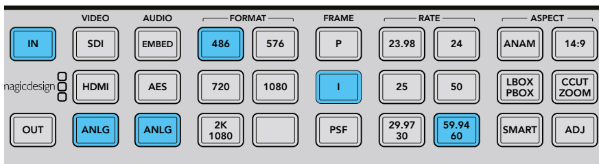
Pressing the IN button displays the input format on the control panel buttons. In the above illustration, the input format is 486i59.94 via analog component with analog audio.
